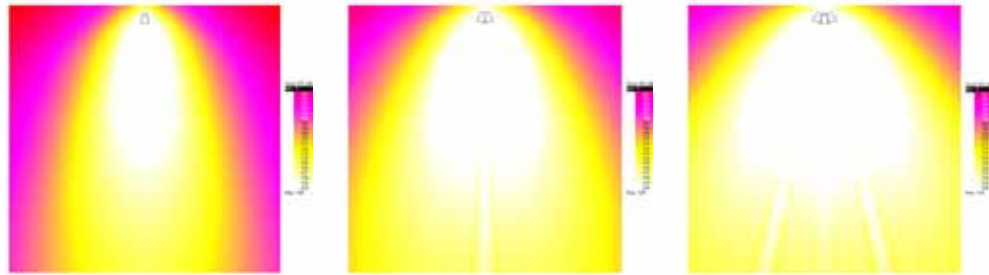
Figure 4.5: Horizontal coverage EDGE212P single, double and triple
