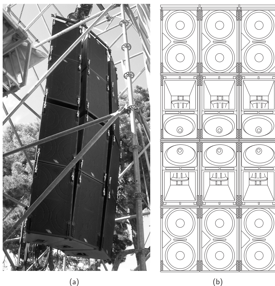
Figure 4.7: EDGE212P and EDGE218SP Array
