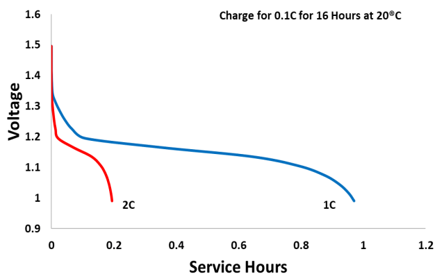
High Rate Discharge- AA Premium
