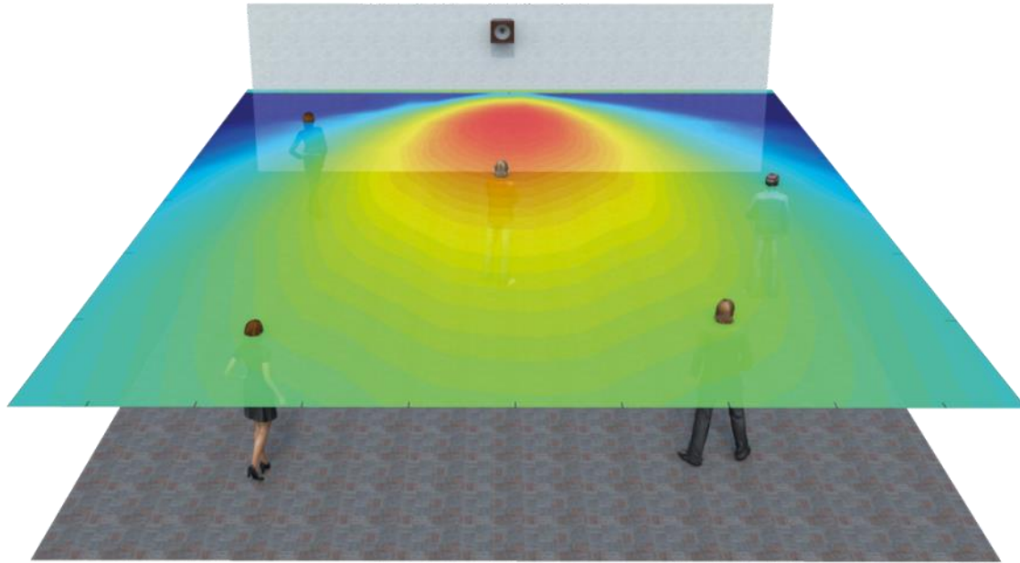
Conventional 2-way loudspeaker coverage
