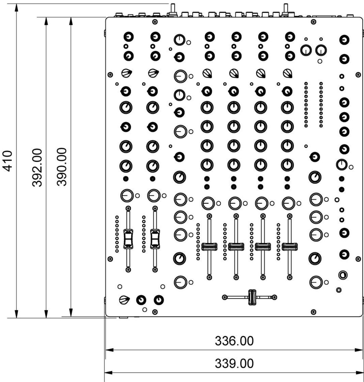
Top Panel View
