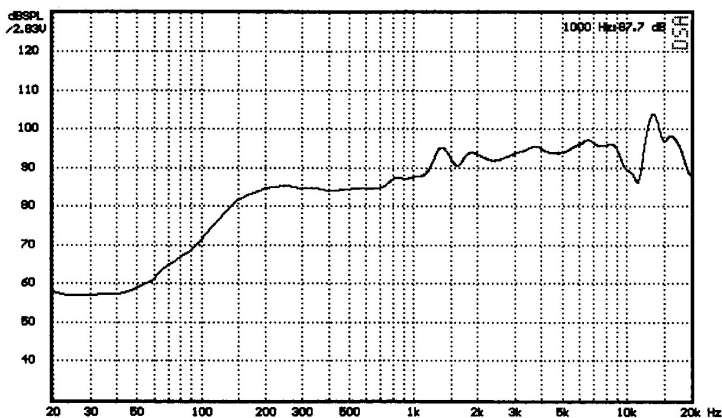
Frequency Response
